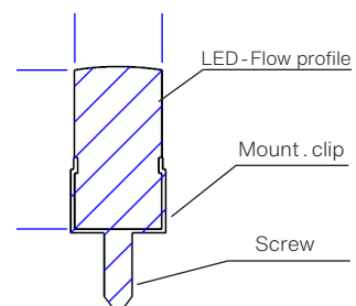
MOUNTING WITH CLIP
